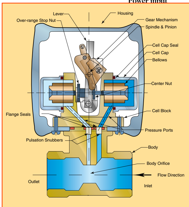
TYPICAL ASSEMBLY OF SERIES 7000 FLO-GAGE
